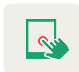
SPARE App
